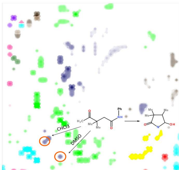
Figure 1. GTM map built for 697 tautomeric equilibria. The color code corresponds to 10 tautomeric classes. Selected data points correspond to the same equilibrium studied in \text{CHCl}_3 ( \log K_T = -0.49 ) and \text{DMSO} ( \log K_T = 0.62 ).
